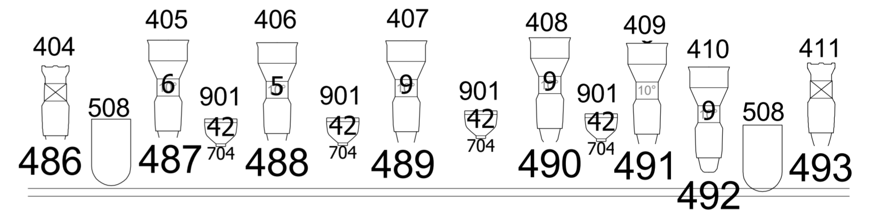
Center Pipe Detail
